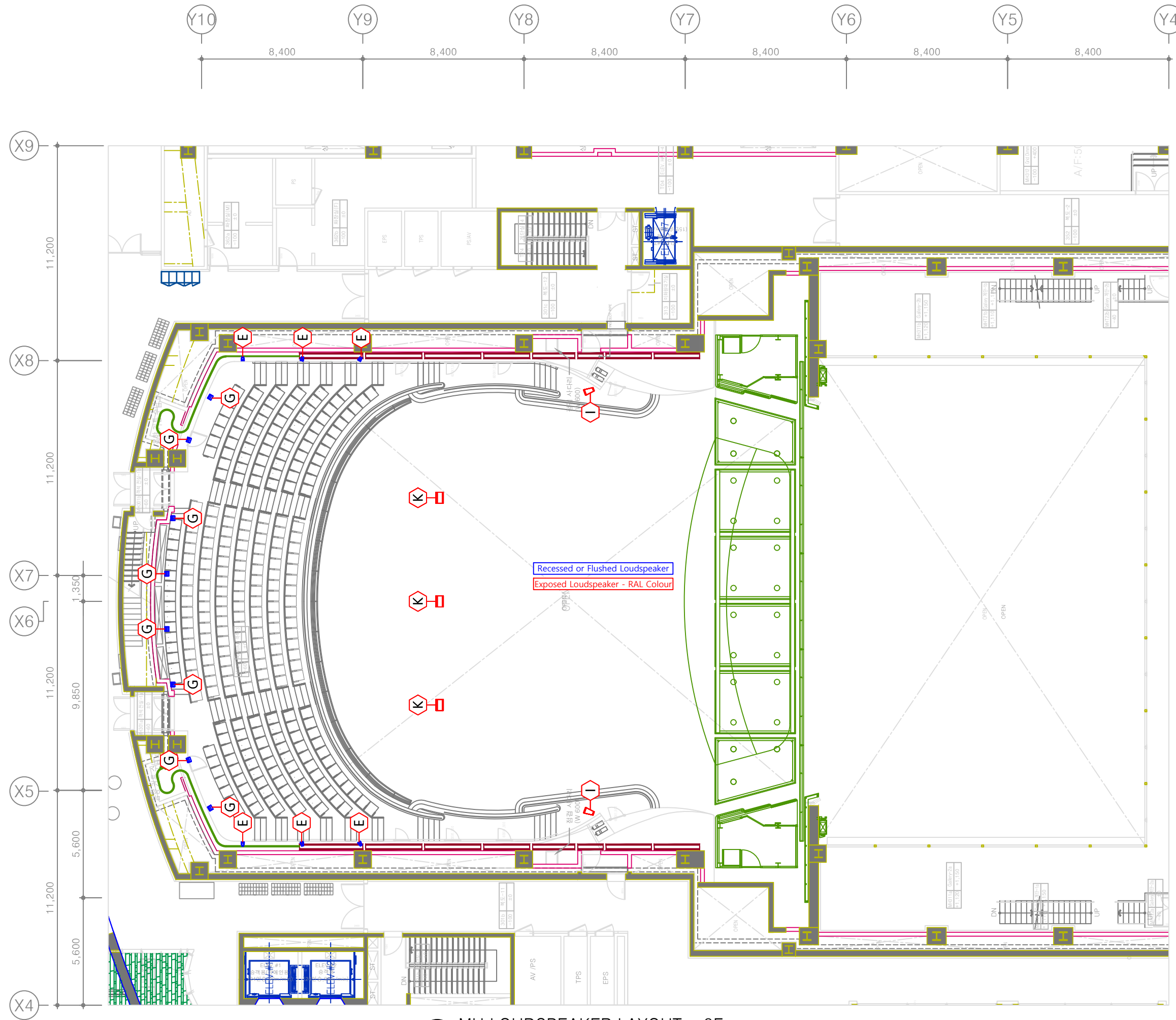
SC MH LOUDSPEAKER LAYOUT - 3F SCALE : 1/100 (A1) SCALE : 1/200 (A3)
