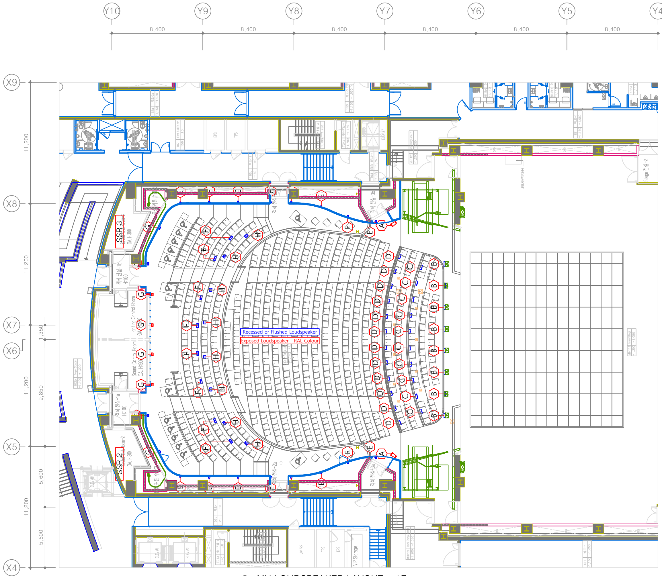
SC MH LOUDSPEAKER LAYOUT - 1F SCALE : 1/100 (A1) SCALE : 1/200 (A3)
