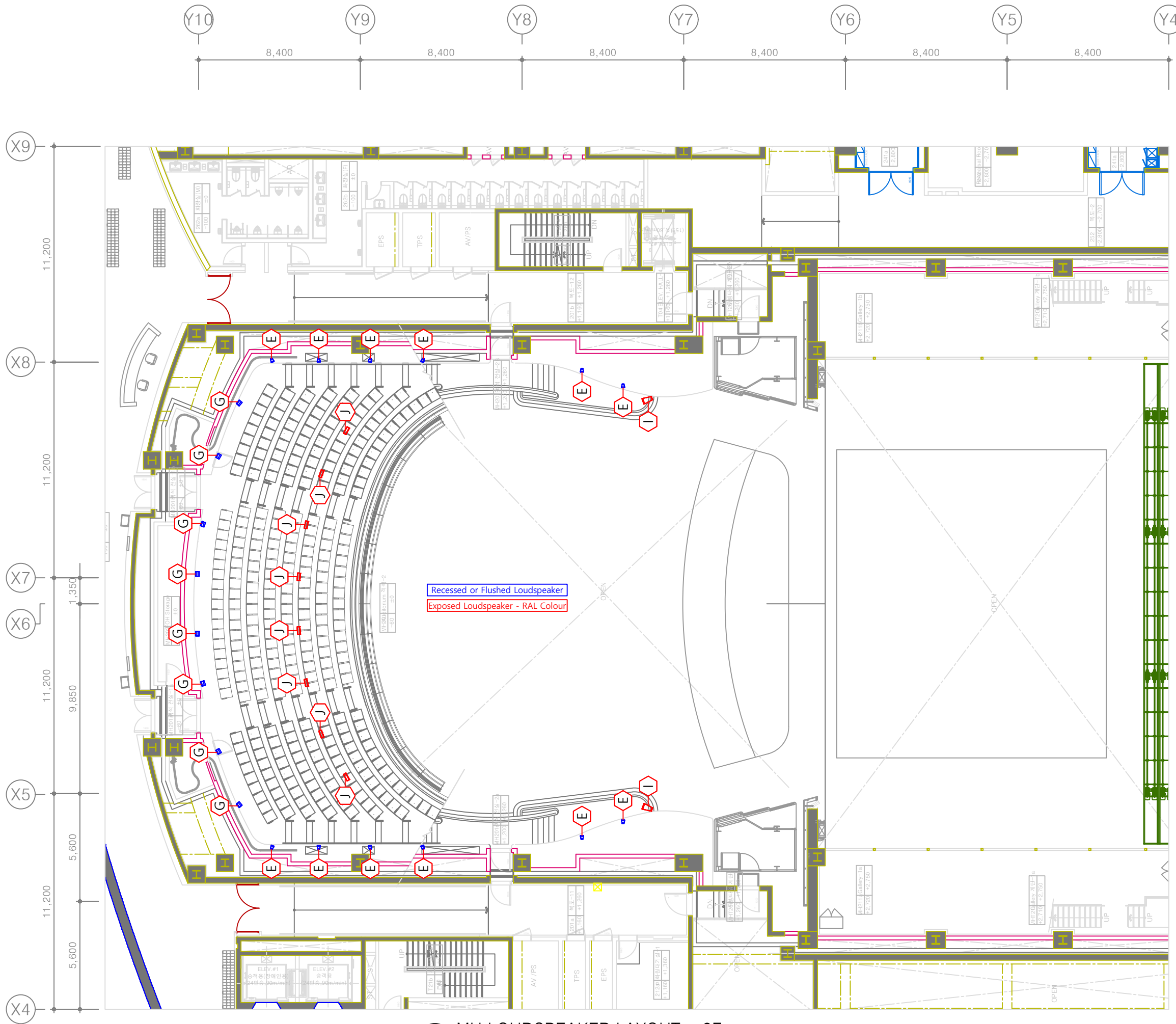
SC MH LOUDSPEAKER LAYOUT - 2F SCALE : 1/100 (A1) SCALE : 1/200 (A3)
